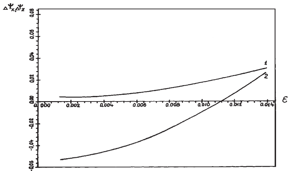
Fig.3 Dependens of the phase shift \nabla\psi_x (1) and \nabla\psi_z (2) of magnitude emittensa beam for a linear coordination (without additional item)
