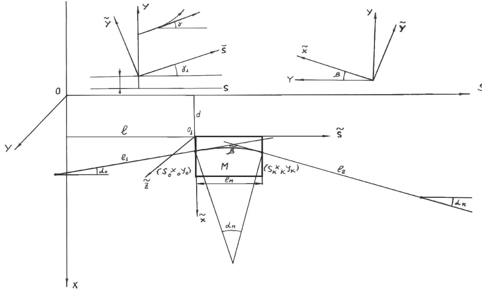
Fig.1 The system of coordinates utilized for calculations: SX– basic rectangular system of coordinates; S_1X_1 and S_2X_2 –systems of coordinates of the 1–st and 2–nd magnets.
