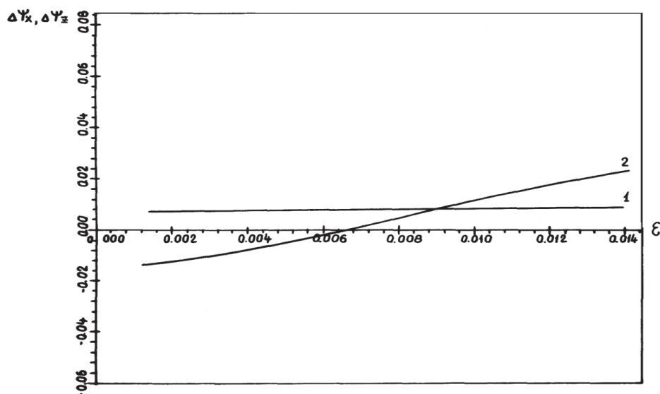
Fig.4 Dependens of the phase shift \nabla\psi_x (1) and \nabla\psi_z (2) of magnitude emittensa beam for a unlinear coordination (with additional item)
