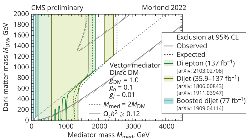
Upper limits at 95% CL on the masses M_{DM} of the Dark Matter particle, which is assumed to be a Dirac fermion, and its associated vector mediator M_{med} , for dijet and dilepton searches from the CMS experiment (LHC Run 2). The painted areas represent the excluded regions
