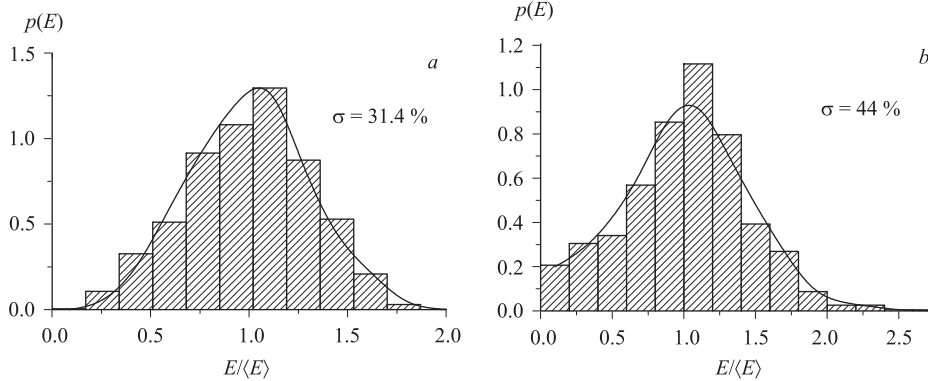
Fig. 6. Probability distributions of the total energy in the radiation pulse ( a ) and after narrow band monochromator ( b ) [2]. TTF FEL operates in the nonlinear regime. Solid lines represent simulations with the code FAST
