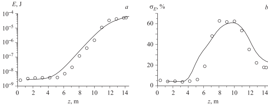
Fig. 2. Energy in the radiation pulse (a) and fluctuations of the energy in the radiation pulse (b) versus undulator length. Circles are experimental data [1], and curves represent results of simulations with the code FAST
