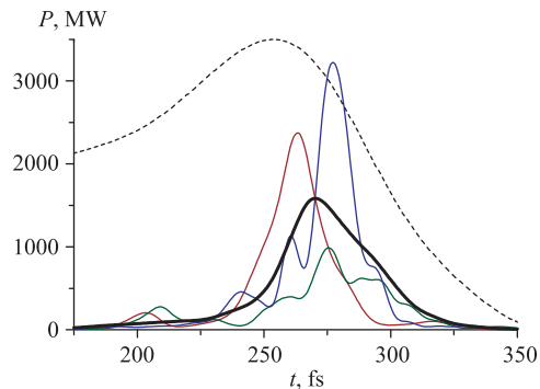
Fig. 7. Radiation power along the bunch for TTF FEL operating in the nonlinear regime. Thin curves represent single shots; bold curve, averaged profile; dashed curve, profile of electron bunch. Simulations are performed with the code FAST
