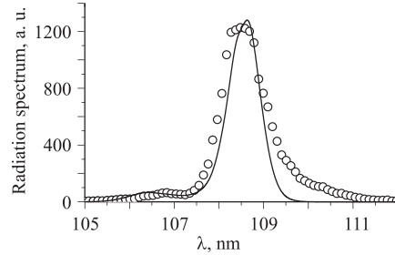
Fig. 3. Average spectrum of TTF FEL operating in the high-gain linear regime. Circles are experimental data [8], and the curve represents results of simulations with the code FAST
