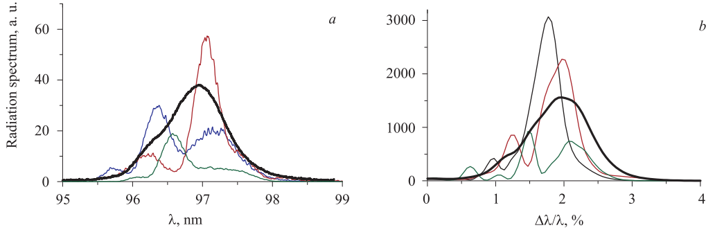
Fig. 4. Single-shot spectra (thin lines) and averaged spectrum (bold lines) of TTF FEL operating in the nonlinear regime: a ) experimental data [1]; b ) results of simulations with the code FAST
