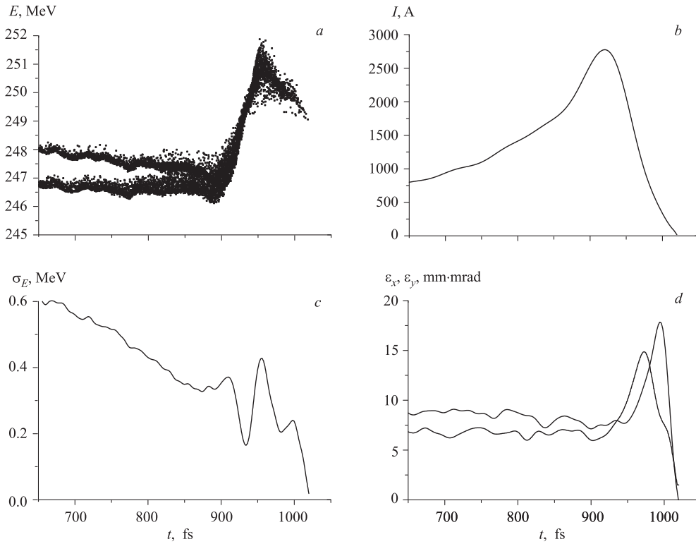
Fig. 1. Longitudinal phase space (a), current (b), slice energy spread along the bunch at the undulator entrance (c) and slice emittance (d). Bunch head is at the right side
