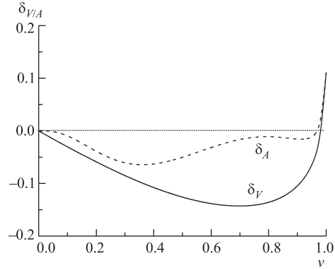
The relative corrections \delta_{V/A} vs. v
