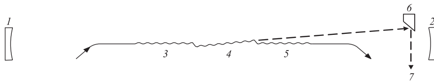
Fig. 3. Scheme of the electron outcoupling for the second stage of the Novosibirsk FEL. 1, 2 — mirrors of optical resonator; 3–5 — undulators; 6 — 45-degree mirror; 7 — radiation output
