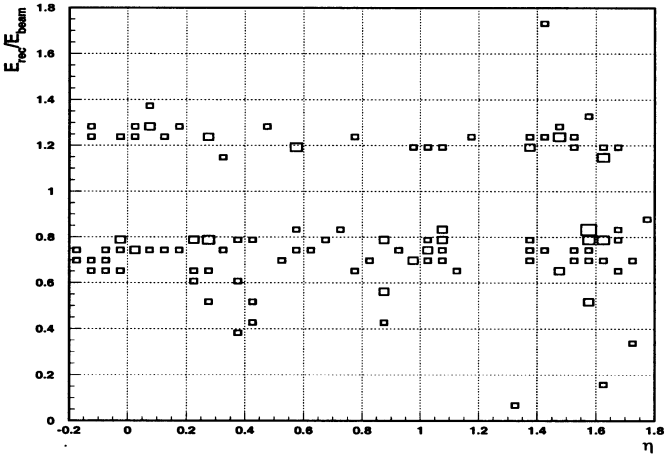
Figure 7: Events in the tails of the distribution of the reconstructed energy as a function of pseudorapidity for pions of E_T = 20 GeV (top plot) and E_T = 50 GeV (bottom plot). Tails are defined as events with reconstructed energies more than three standard deviations away from the mean.
