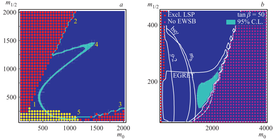
Fig. 1. a) MSSM parameter space. Light blue line corresponds to the region consistent with WMAP data. One can distinguish between different regions marked by digits. 5 — is the EGRET region. b) The light shaded (blue) area is the enlarged region preferred by EGRET data for \tan \beta = 50 , \mu > 0 and A_0 = 0 . The excluded regions where the stau would be the LSP, or the electroweak symmetry breaking fails, or the Higgs boson is too light, are indicated by dots
