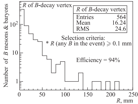
Fig. 6. The free path of B hadrons created in the process (1) before their decay. The criterion for the event selection is that the free path is not less than 100 \mu\text{m} for each of four B hadrons in the same event. 94% of events satisfy this condition
