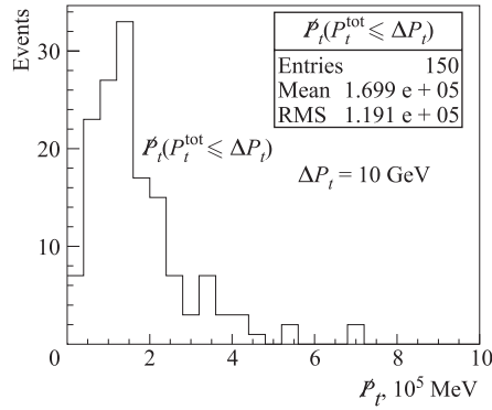
Fig. 5. Total missing transverse momentum P_t of two neutralinos. Event selection is made assuming that the total P_t of gluino pair is less than 10 GeV. Since in our study the initial state radiation was not taken into account, all events satisfy this condition
