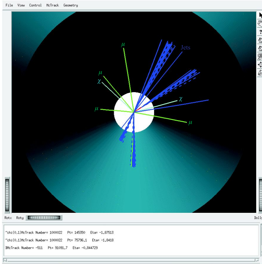
Fig. 3. Generation of the process 1 inside the cylindrical (Layer 1) pixel detector in the XY plane (transversely to the beam). One can see four muon tracks (green lines), two tracks from neutralino (light blue lines), four jets (dark blue lines) and one long-living B meson (red line). Visualisation has been performed with the help of ATLAS GeoModel HitDisplay [8]
