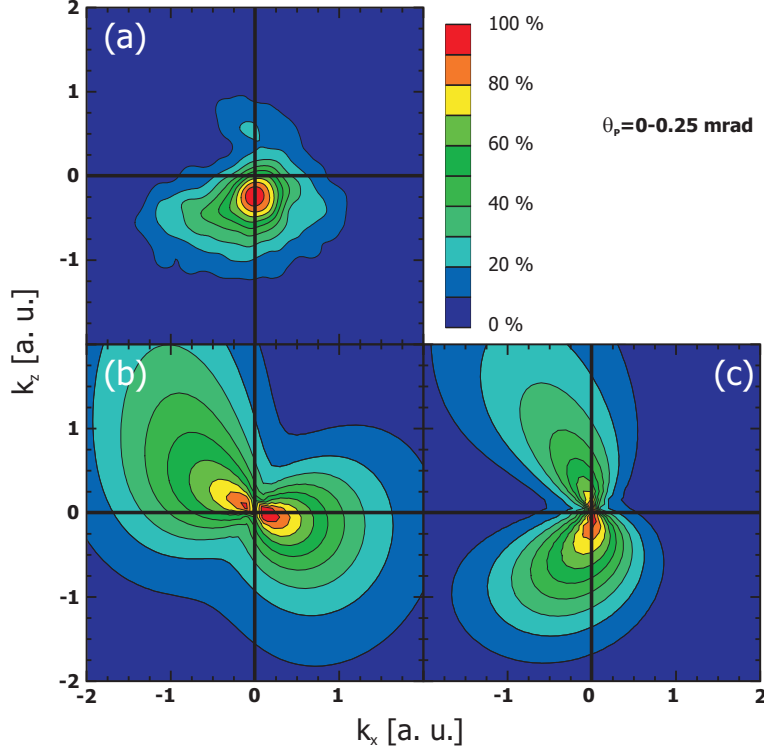
FIG. 2: Experimental and theoretical data for 630 keV H + /He collisions for \theta_p \leq 0.25 mrad. (a) are the experimental data and the red dashed line represents the binary encounter ridge. (b) calculations using a helium 1s^2 trial wave function, while (c) uses a highly correlated helium wave function with angular momentum, all including terms A_1 + A_2 + A_3
