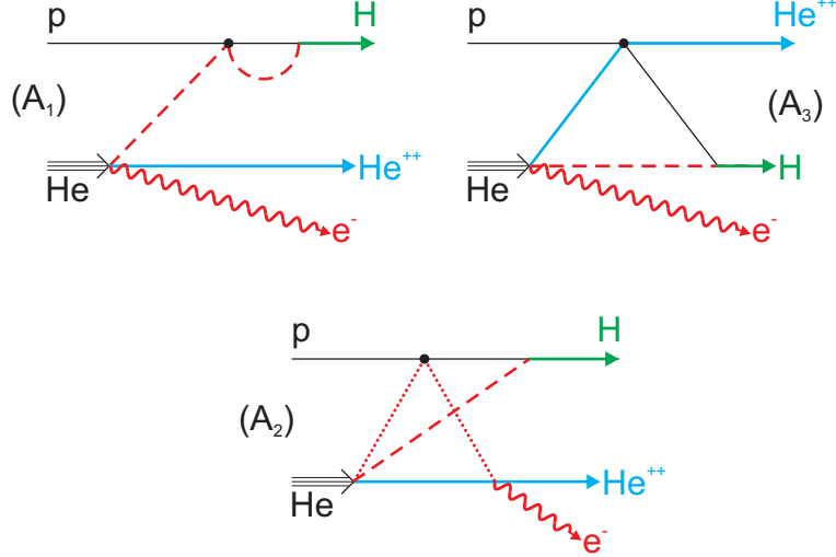
FIG. 1: Schematic presentation of non-symmetrized A_1 + A_3 and A_2 terms. A_1 (OBK) describes the collision between electron and proton followed by the capture of this electron by the projectile. The second electron is released due to rearrangement in the helium, known as shake-off (SO). The A_3 amplitude represents first an interaction between the projectile and the helium nucleus followed by electron capture. Similarly to A_1 the second electron is also released due to the sudden rearrangement in the helium. Term A_2 describes the classically termed TS2 amplitude. First the proton knocks-off a target electron into the continuum, followed by capturing the remaining electron from the helium.
