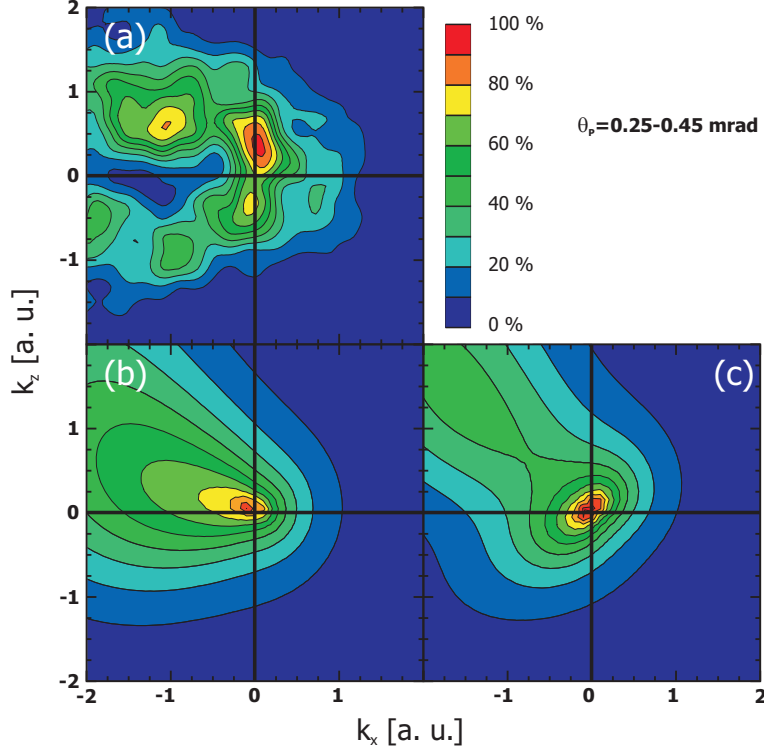
FIG. 4: The same like in Fig. 2, but for 0.25 \leq \theta_p \leq 0.45 mrad.
