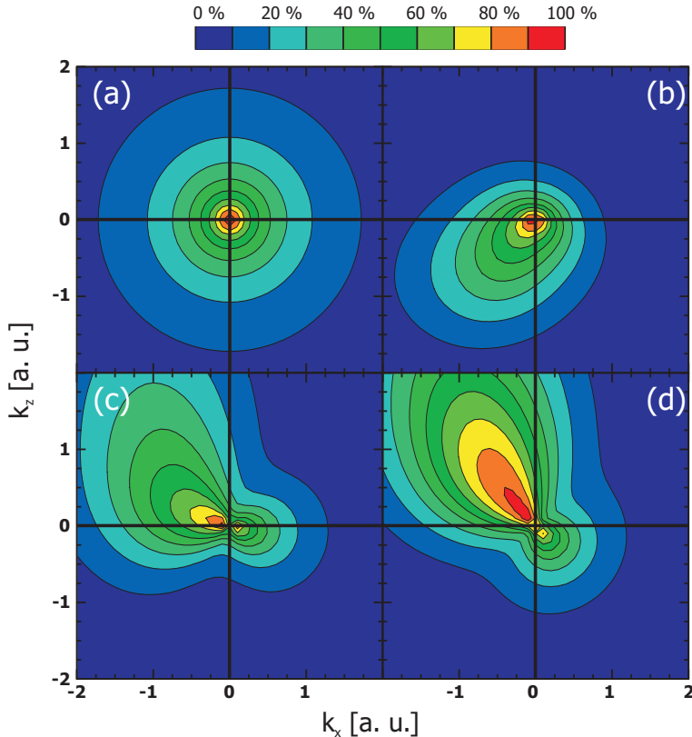
FIG. 3: Calculations for \theta_p \leq 0.25 and helium 1s^2 trial wave function separated in SO (a) and TS2 (c) contributions. Similar calculations for highly correlated helium wave function are presented in panels (b) and (d).
